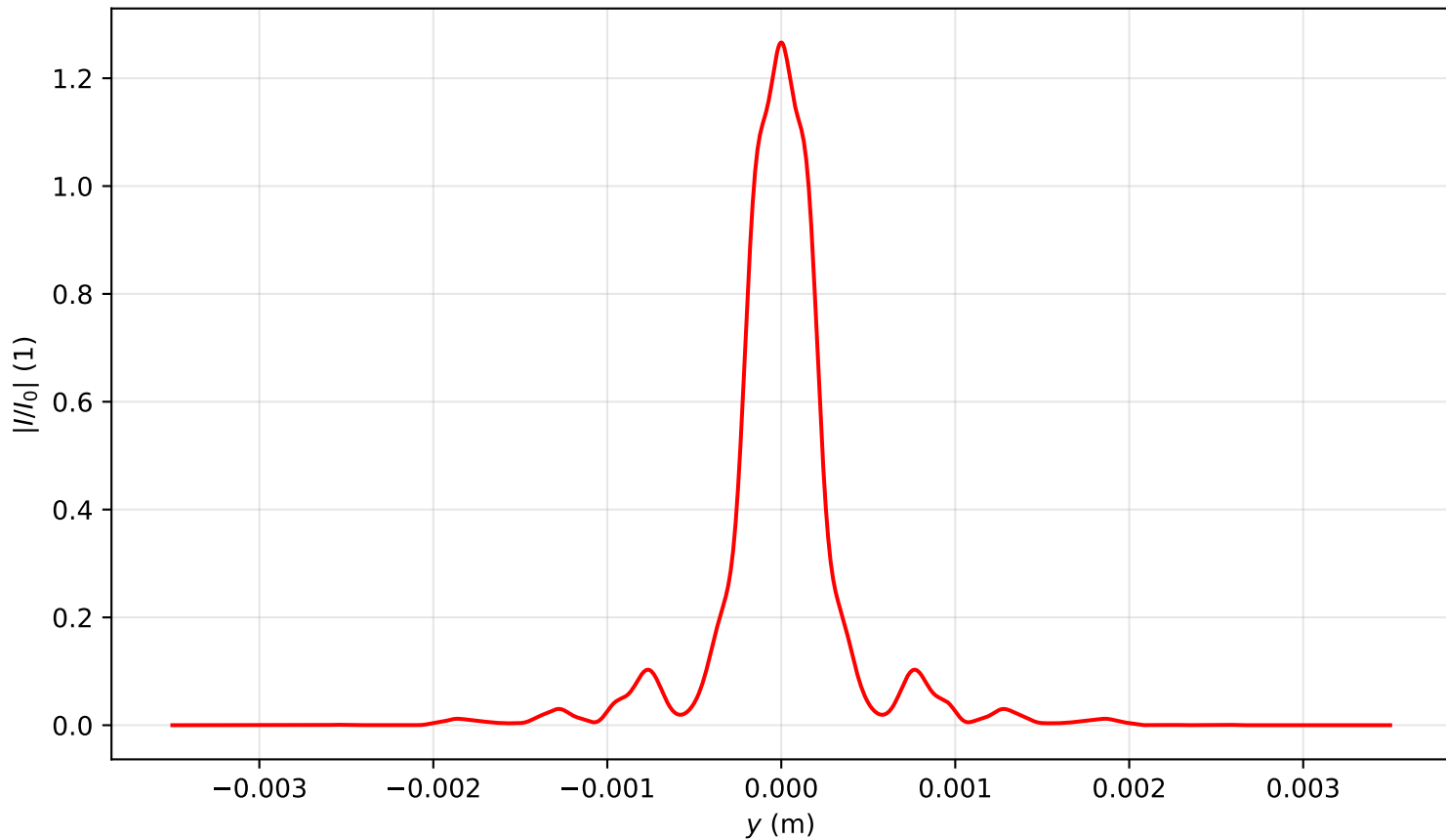
Intensity profile I(x = 0, y, z = 1.672)/I_0 , \text{Pin}=5.5\text{Pcr} , artificial time
